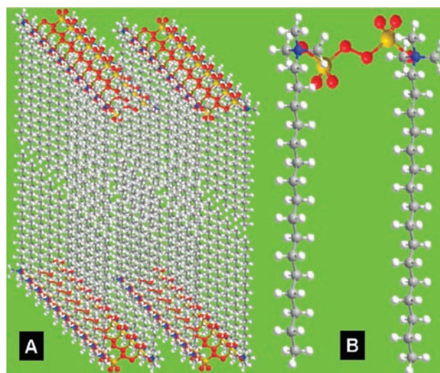
Scheme 1. (A) Lamellar Structure of the (CTA)_2S_2O_8 Complex Micelle and (B) Individual (CTA)_2S_2O_8 Complex with Protonated Monomer a
